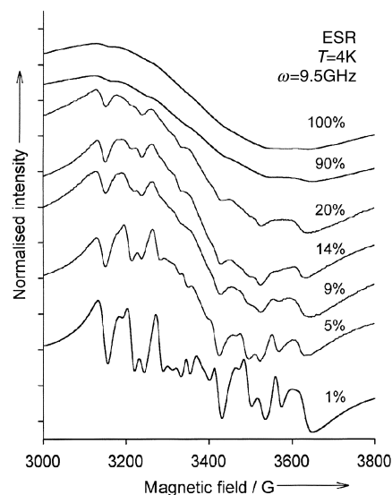
Figure 13. Normalised EPR spectra of seven host–guest compound powder samples of different Mn contents x at T = 4 K.
